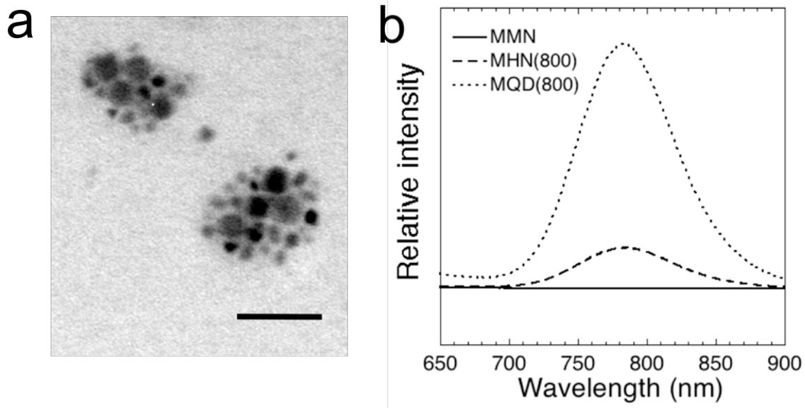
Figure S5. (a) TEM image of MHN composed of MN and QD emitting at 800 nm [MHN(800)]. Scale bar is 50 nm. (b) Photoluminescent spectra of MMN, MQD(800), and MHN(800), obtained with 450 nm excitation.
