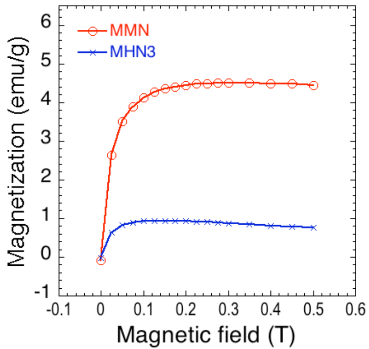
Figure S1. SQUID magnetization curves for MMN and MHN3 samples. The magnetization values are normalized by the total mass of particles in each sample.
