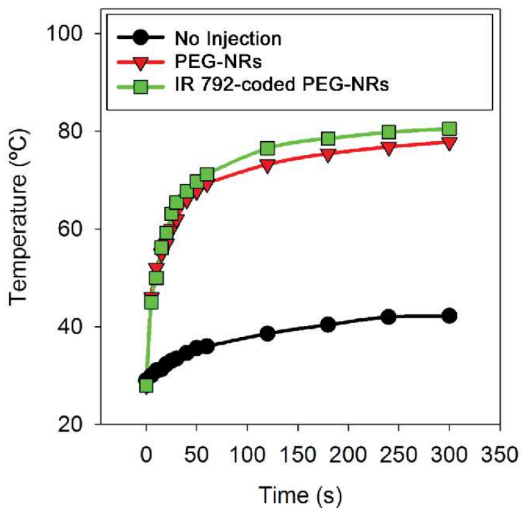
Figure 4S. Photothermal heating of xenograft tumors in vivo following intratumoral injection. Athymic (nu/nu) mice were intratumorally injected with SERS-coded- or unlabeled PEG-nanorods (20 femtomoles each) and irradiated with an 810nm diode laser source ( 2\text{W}/\text{cm}^2 , 5 min) while under anesthesia. Infrared thermography was utilized to track maximum tumor temperatures over time following the onset of irradiation with comparison to a control tumor lacking nanorod antennas.
