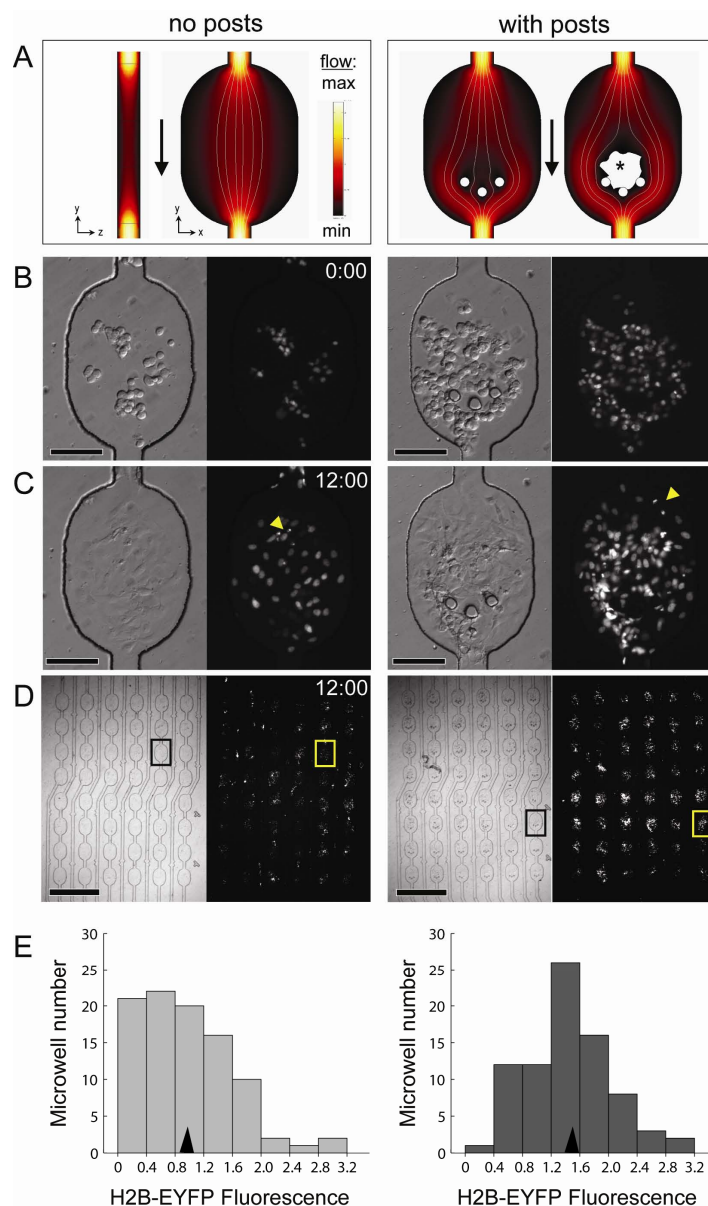
Supplemental Figure 2. Microwell design affects cell loading. (A) Flow simulations (velocity and streamlines) demonstrate decreased flowrate in the center of each microwell. The presence of catching posts (right) further decreases fluid flow in the center of the channel, but allows flow around captured cells (*) to load downstream microwells. Arrows indicate flow direction. Microwells loaded with identical suspensions of histone H2B-EYFP-labeled PtK2 cells are shown in phase and epifluorescence, immediately (B) and after 12 h (C,D). Arrowheads indicate dividing cells. Cell loading was estimated by integrating fluorescence per well at 12 h post-seeding (E). Catching posts increase seeding efficiency by ~50% (1.47 vs. 0.98 fluorescence units) and well-to-well uniformity; however, subsequent cell attachment and migration up the posts prevented microscopy in a single z-plane. Scale bars: 100 \mu\text{m} (B,C); 1 mm (D).
