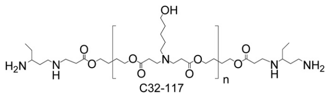
Fig. 1. Polymer structure of C32-117. Ends of the polymer can be in either of the two configurations shown.
