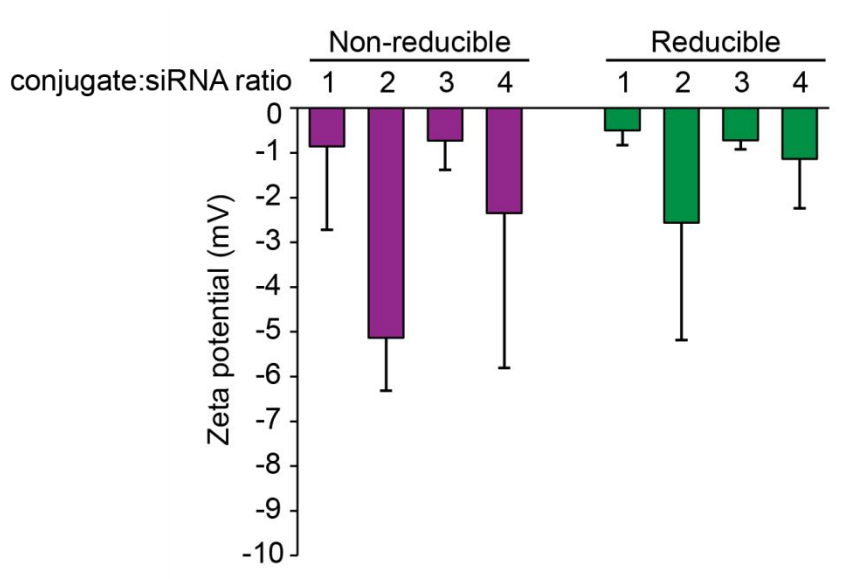
Supplementary Figure S3. Zeta potential measurements of non-reducible and reducible PSNPs at conjugate:siRNA ratios between 1-4.
